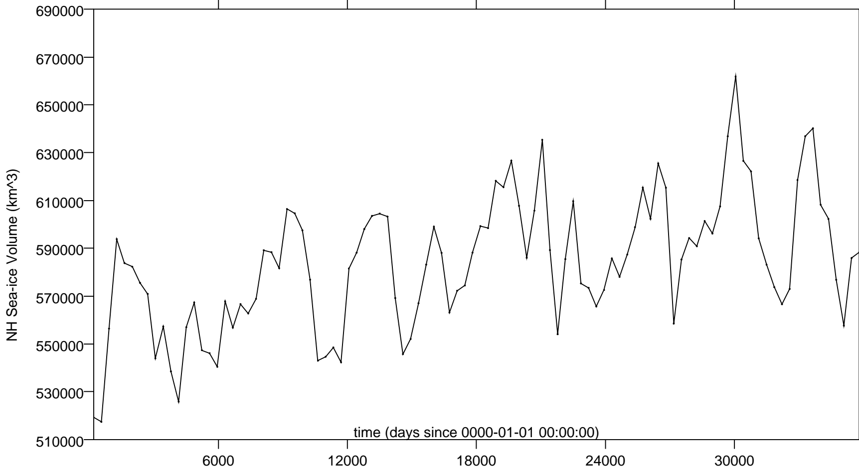
NorthernHemisphere_sea-ice_vol_pmip2_6k_oa
