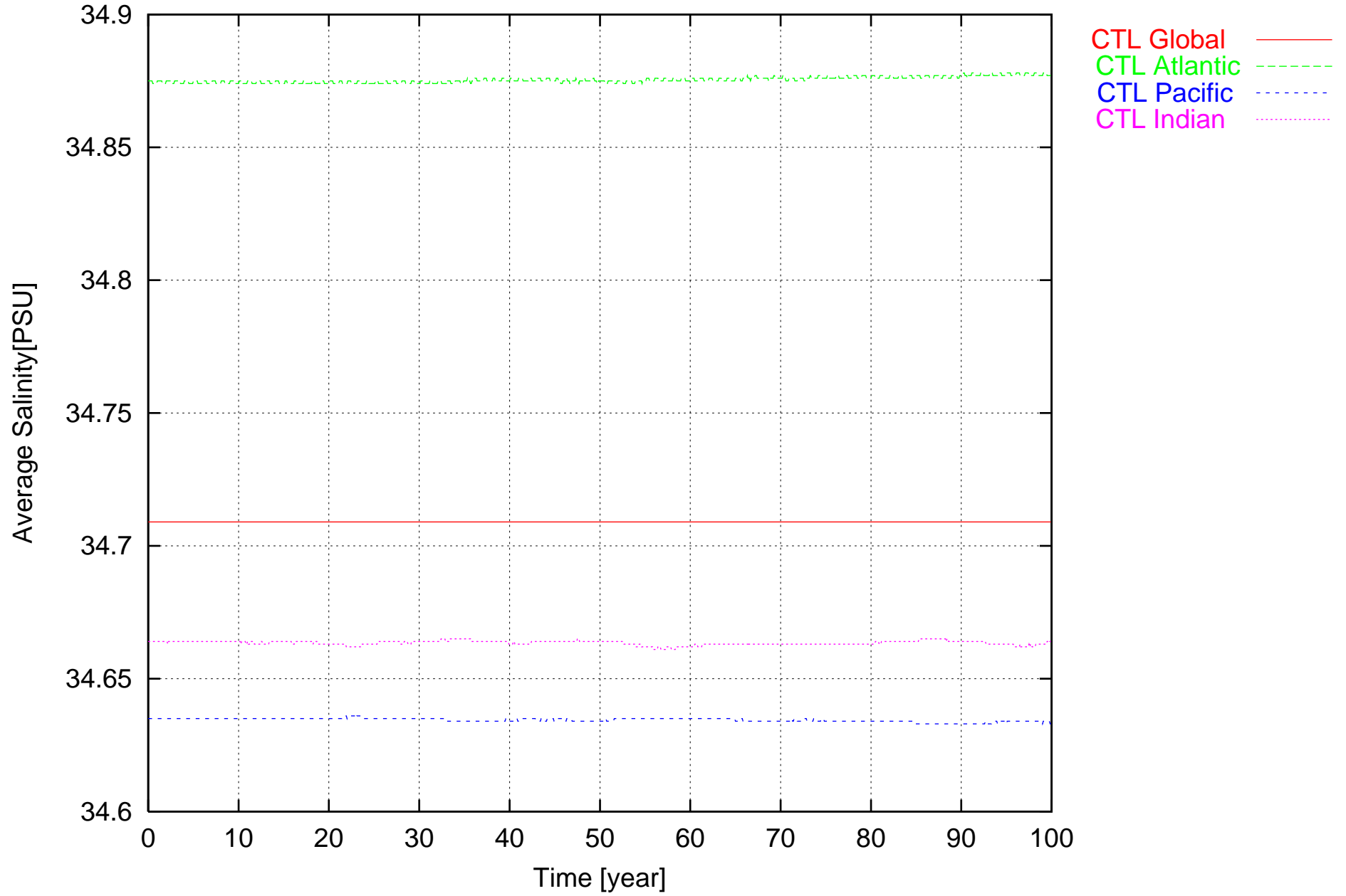
CTL Ocean SSS Trend
