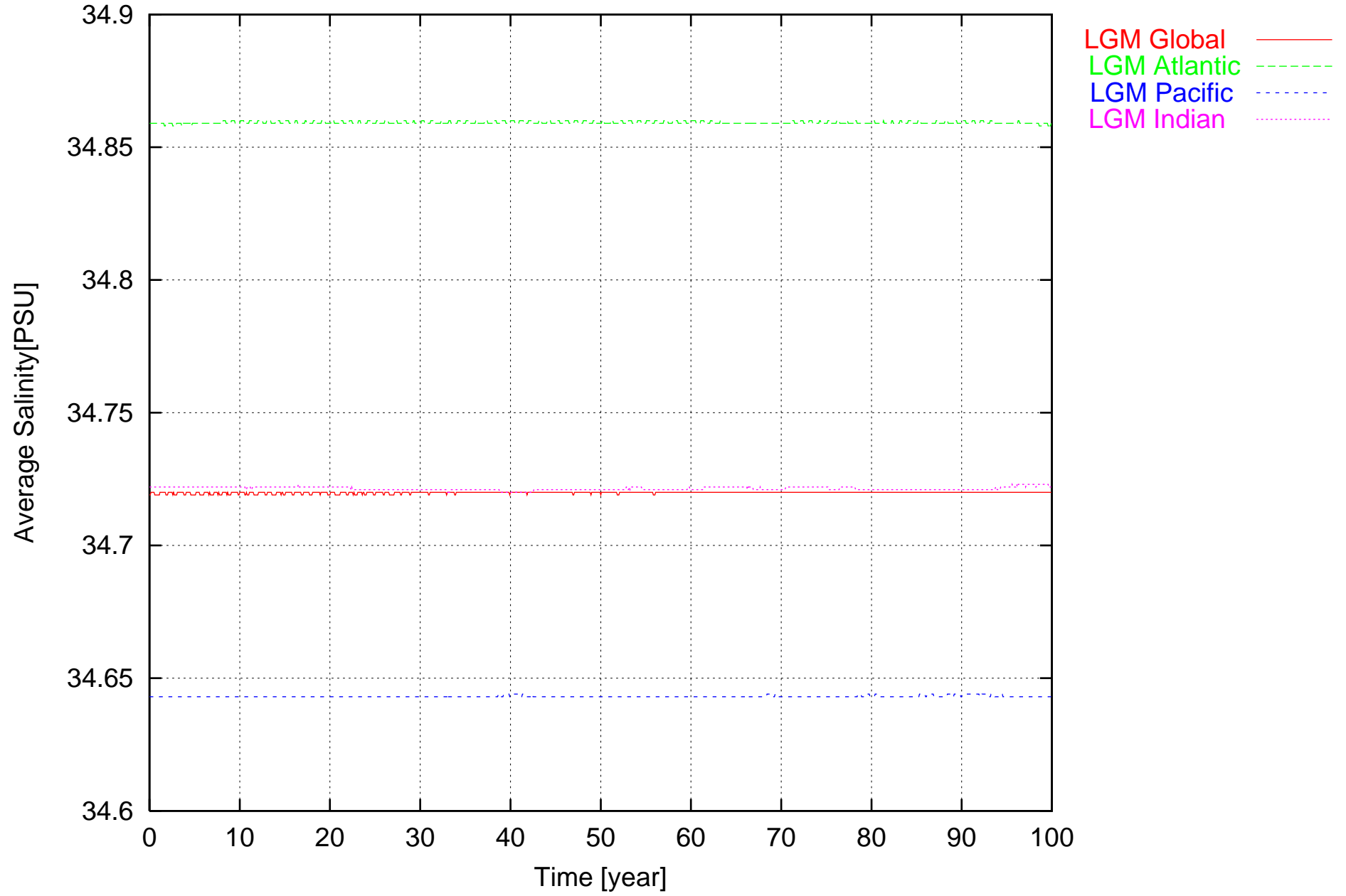
LGM Ocean SSS Trend
