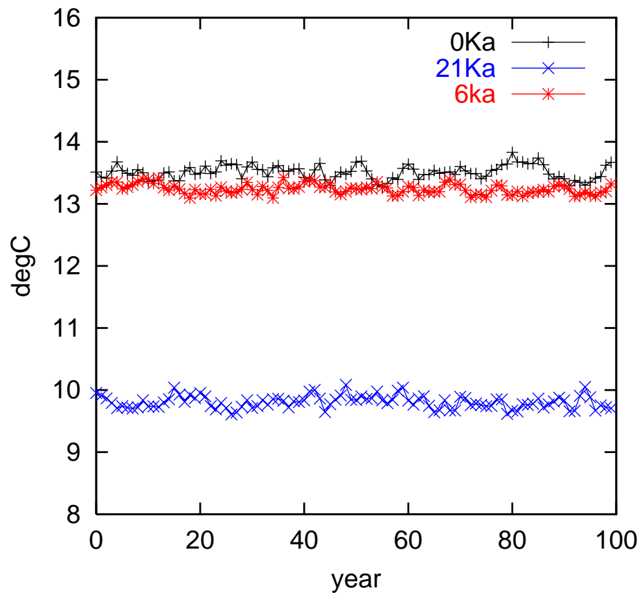
tas time series
