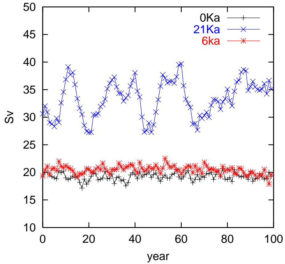
NADW index time series
